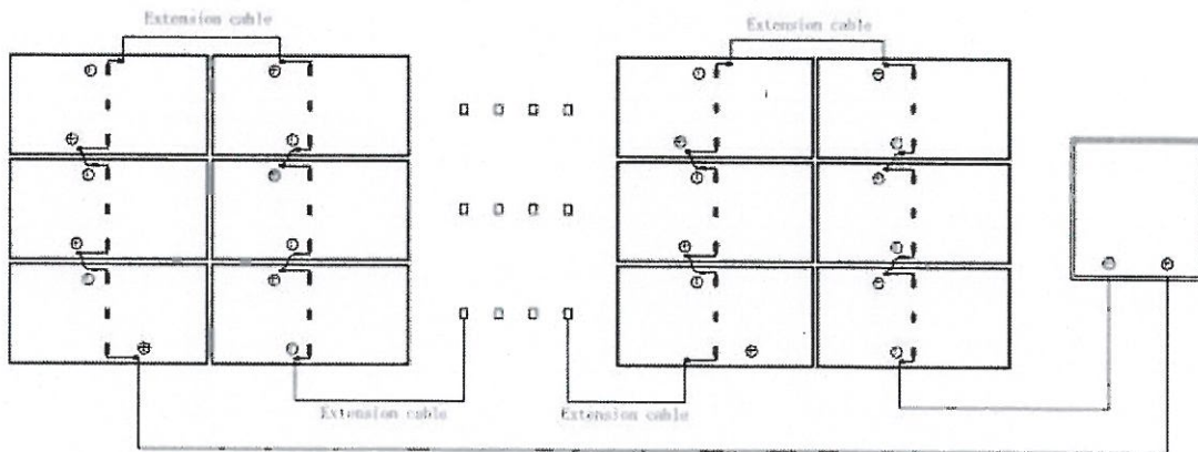
Fig. 5-6 Split J-Box at module middle position for horizontal direction
