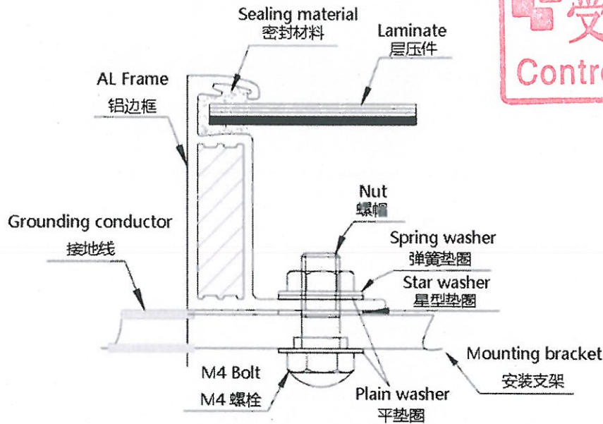
Fig. 5-8 Grounding Diagram
